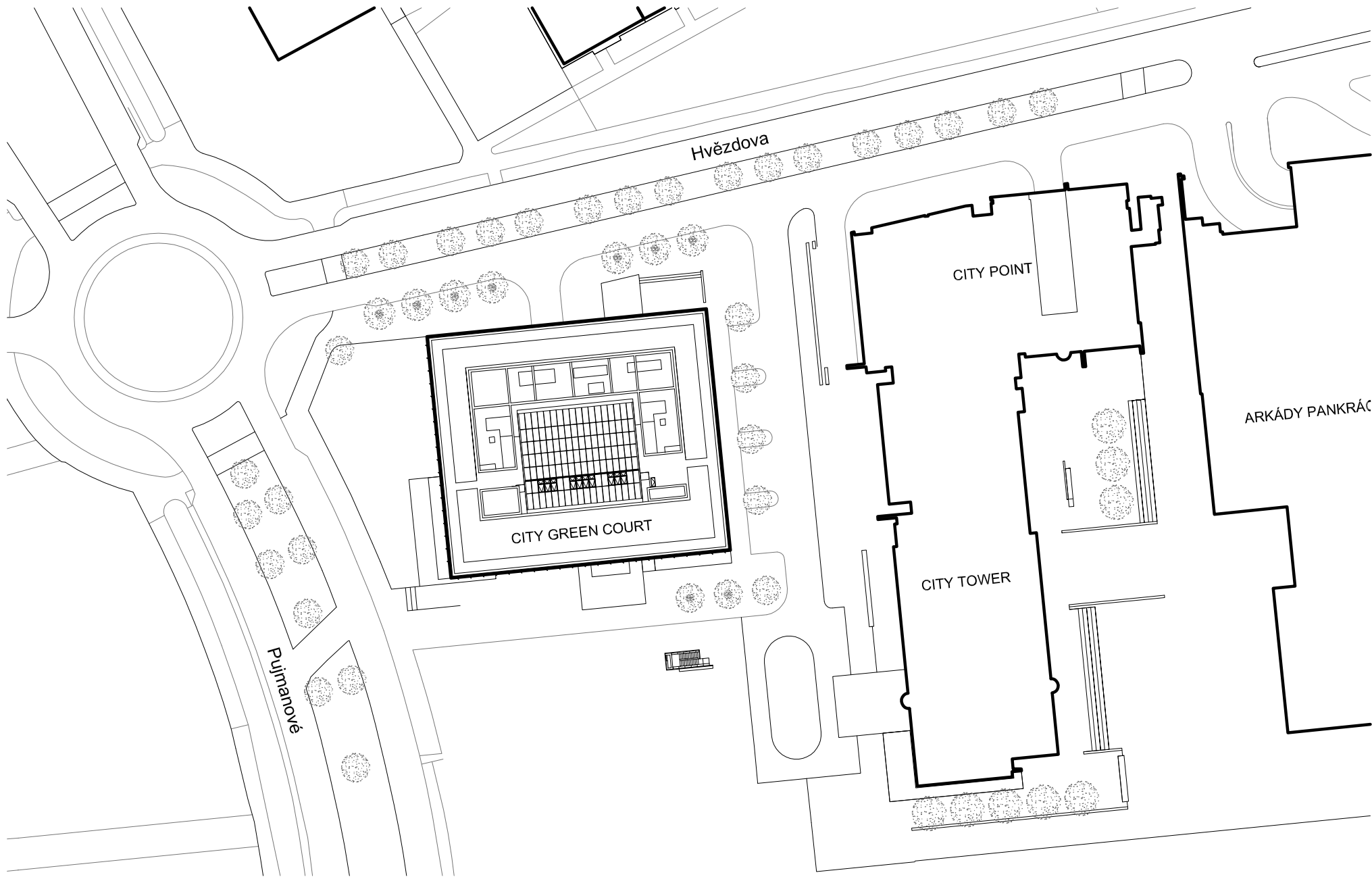
CITY GREEN COURT SITUACE 1:1000
